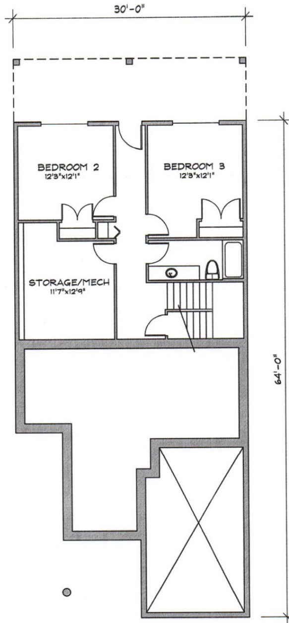
BASEMENT FLOOR PLAN 548 SQ.FT.
